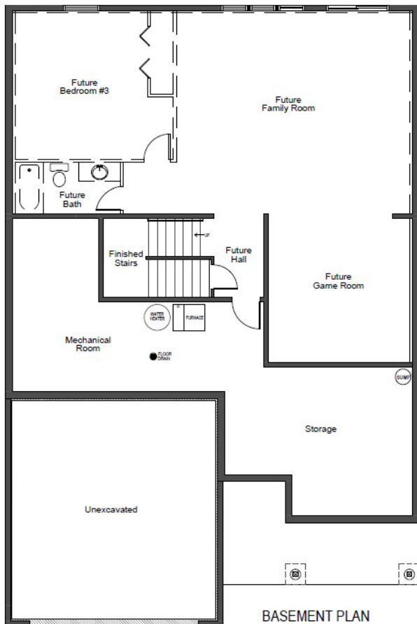
BASEMENT PLAN
